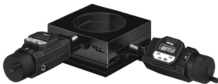
Optional: Co-ordinate table MA 143-6 (50 x 50 mm) with DIGIMATIC digital micrometer heads
